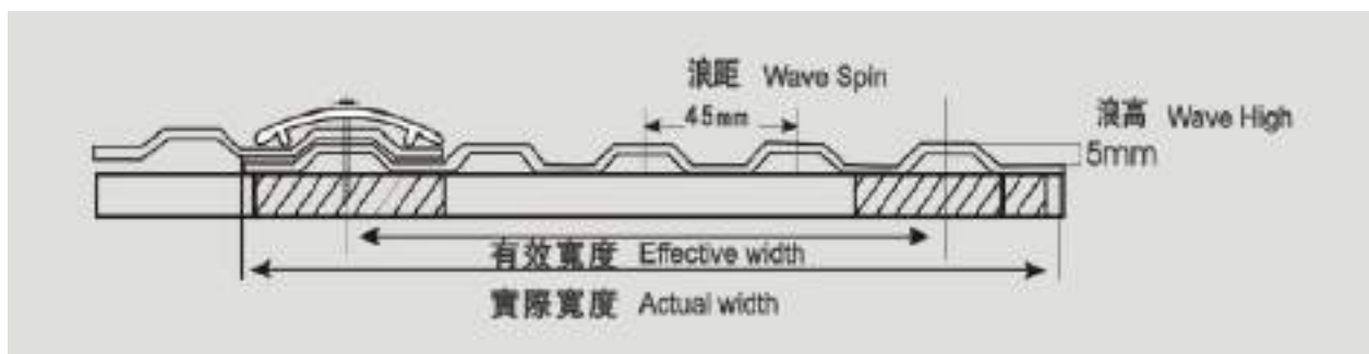
Section of Soflrite polycarbonate corrugated sheet
